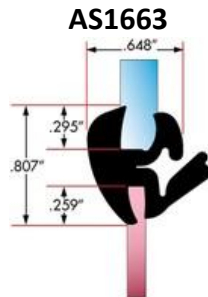
AS1663 75000803, AS-1663 Self-Locking Weather-strip
