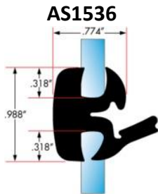
AS1536 1/4 to 1/4 Self Locking Strip 50'
