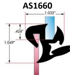
AS1660 75000602, AS-1660 One-Piece Weather-strip 50'
