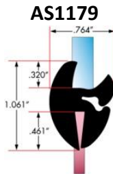
AS1179 Interlocking Universal Weather-strip
